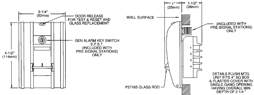
FLUSH INSTALLATION USING P-024900 STEEL BOX
