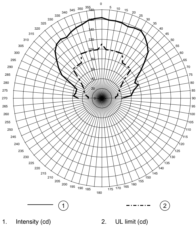
Figure 5: Typical horizontal light output profile, 110 cd setting
