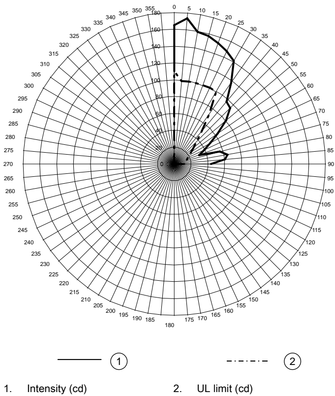
Figure 6: Typical vertical light output profile, 110 cd setting
