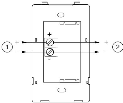
Figure 2: Wiring diagram
